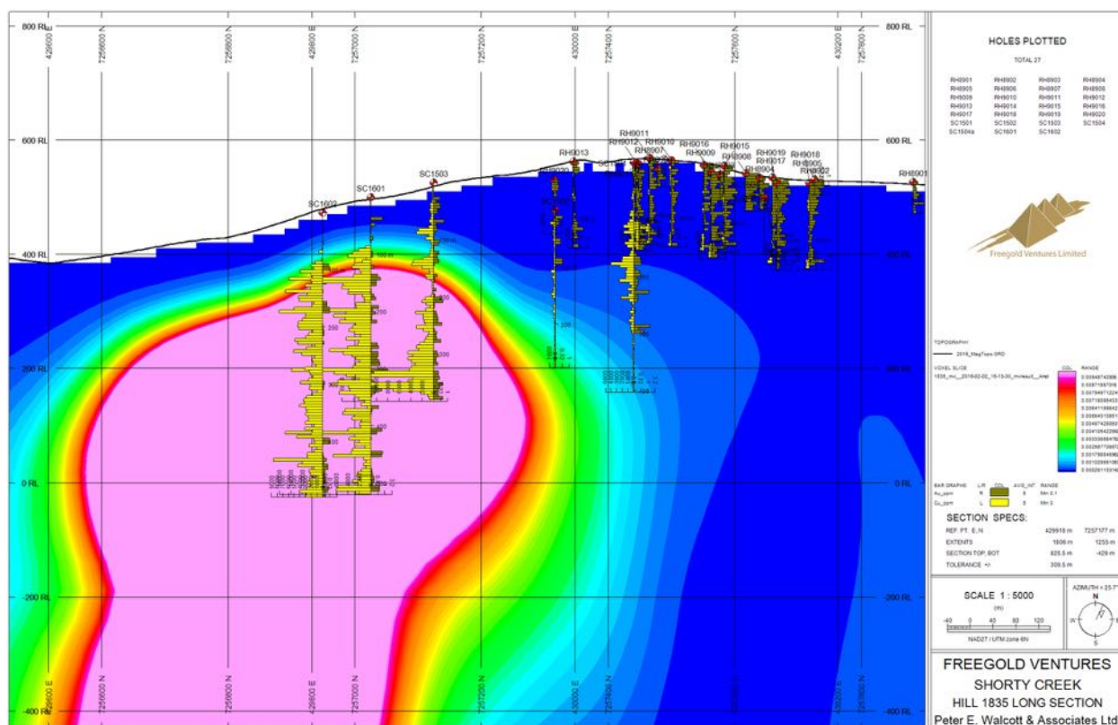
Figure 10.2.3 Cross Section SC 16-01 and SC 16-02 on Magnetic Model Hill 1835 Area
