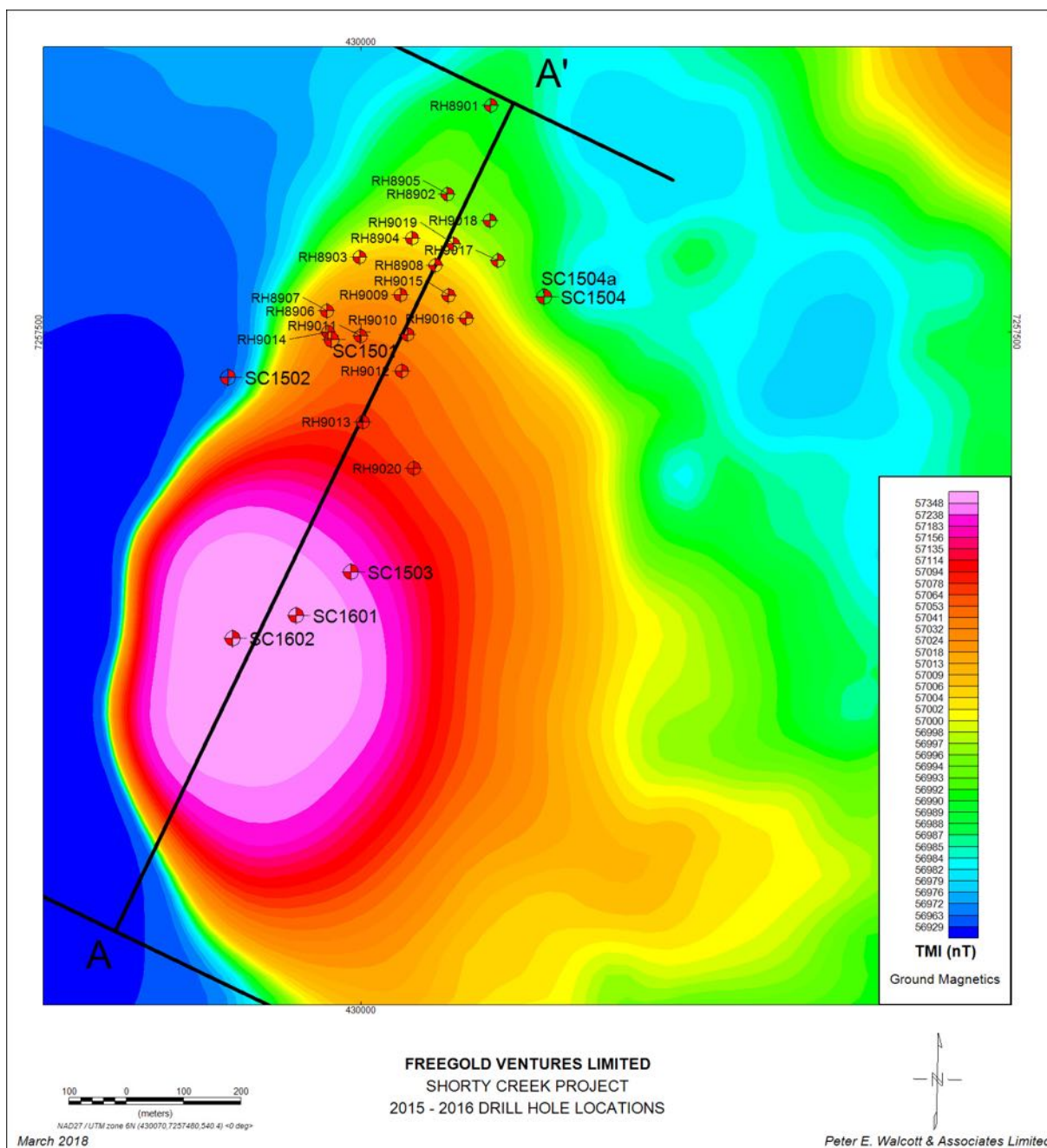
Figure 10.2.2 Location of SC 16-01 and SC 16-02 Hill 1835 Area showing trace of composite section
