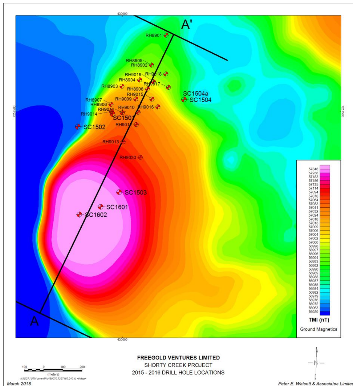
Figure 10.1.1 Map Showing 2015 and 2016 Drill Hole Locations on Hill 1835 and trace of composite section
