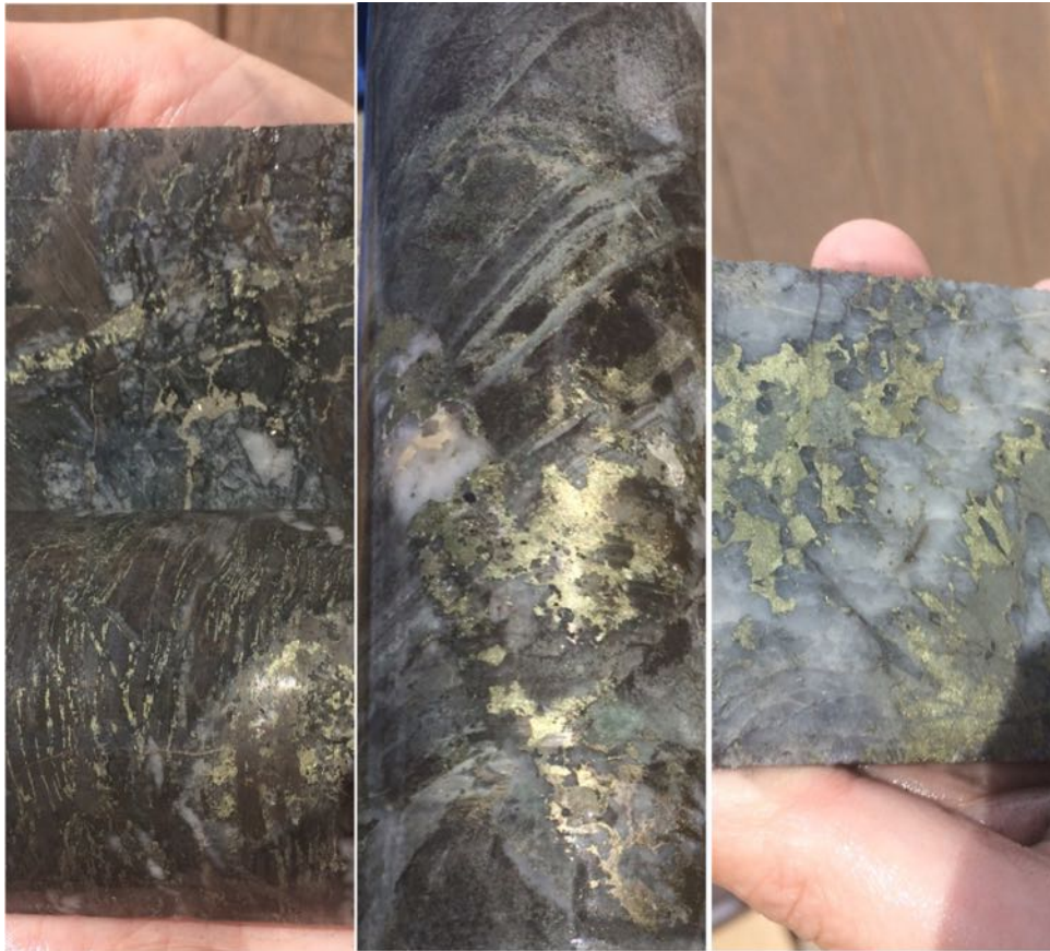
Figure 10.3.3 Copper Mineralization
