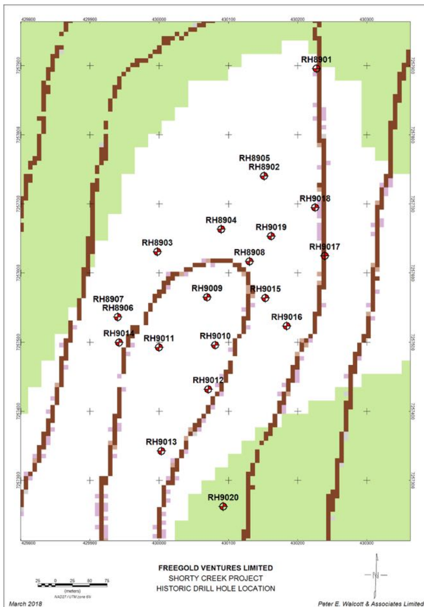
Figure 6.1 Map Showing Historical Drill Hole Locations Hill 1835
